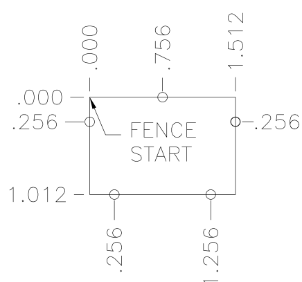
1.0" Pin Pattern
