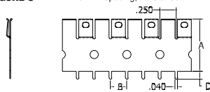
FIGURE 8 .25" Pin Spacing, No Standoff
