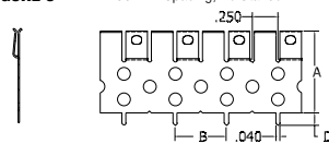
FIGURE 9 .50" Pin Spacing, No Standoff
