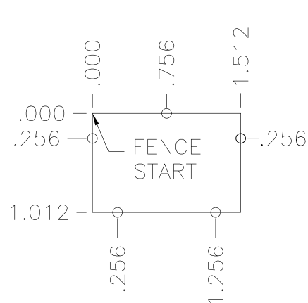
1.0" Pin Pattern
