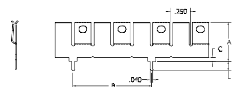
FIGURE 6 .25" Pin Spacing, No Standoff
