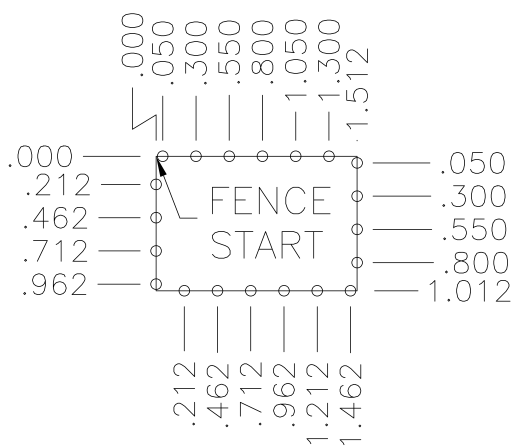
.25" Pin Pattern
