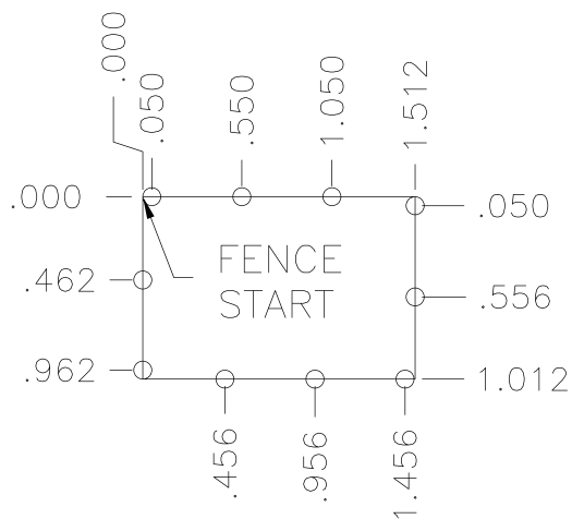
.50" Pin Pattern
