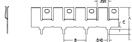
FIGURE 4 1.0" Pin Spacing, No Standoff
