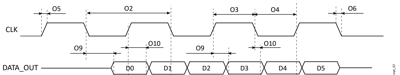
Figure 5-15 OSPI Timing Diagram - DDR Mode (Transmit)
