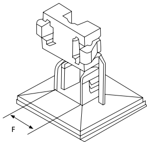
TC349A-TB TC5349A-TB
