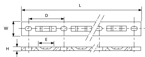
TC1101 ... TC1117
