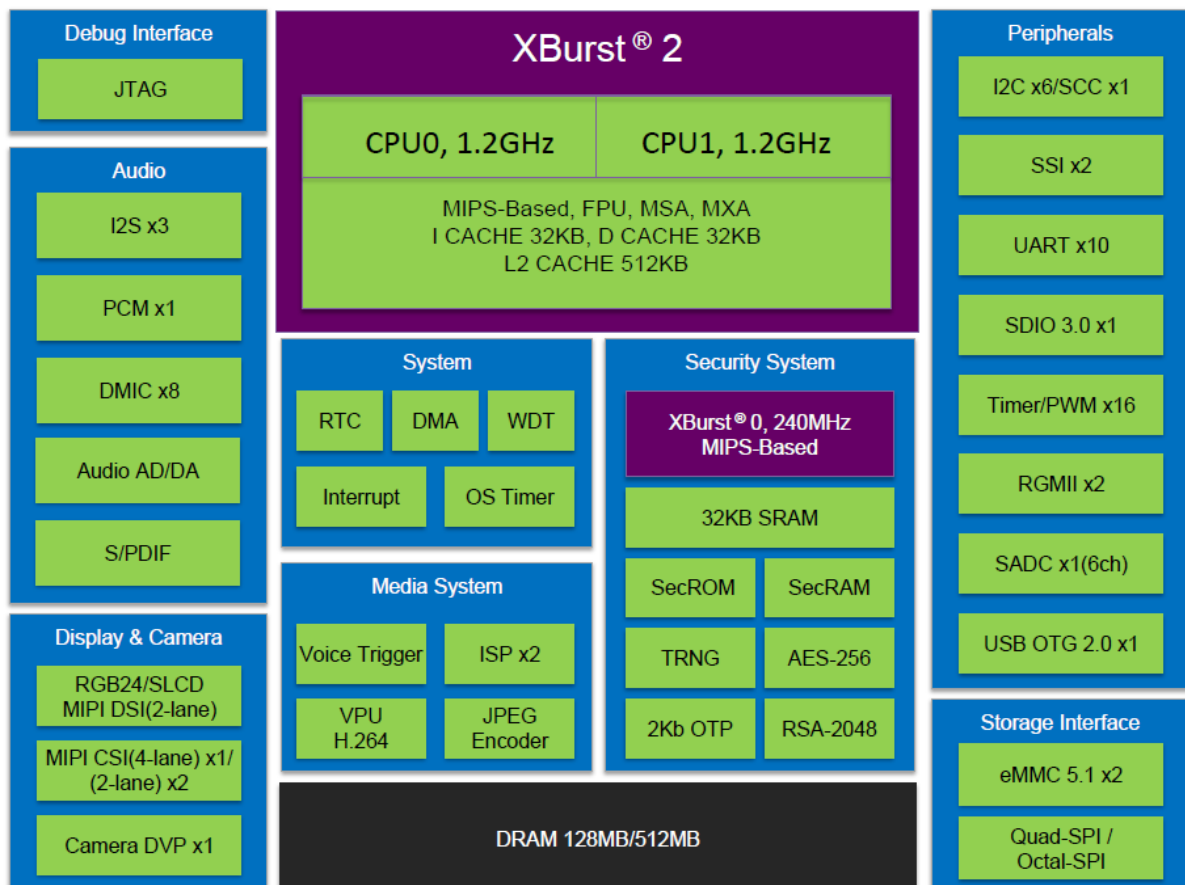
Figure 1-1 X2000/H Diagram
