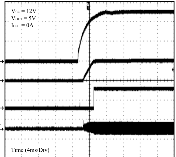
Figure 21 Start Up with VCC
