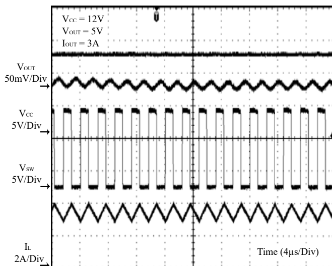
Figure 30 Output Ripple
