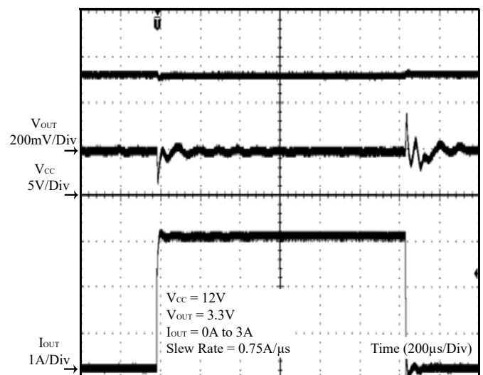
Figure 31 Load Transient
