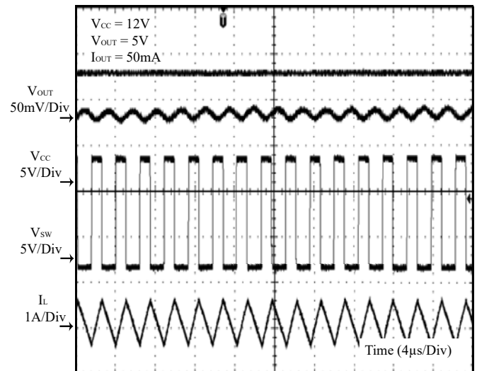
Figure 29 Output Ripple
