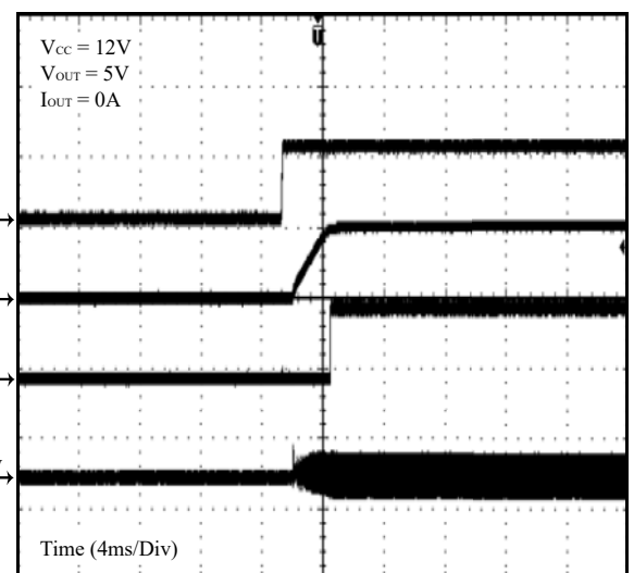
Figure 25 Start Up with EN
