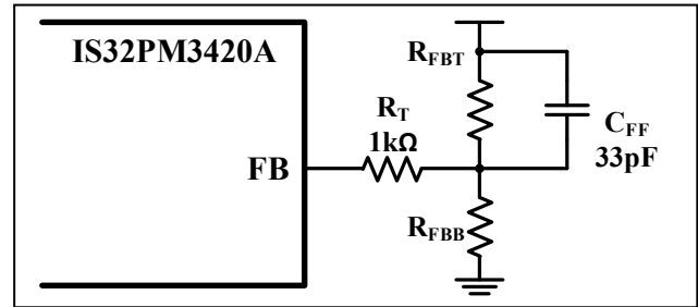
Figure 44 Feedback Network
