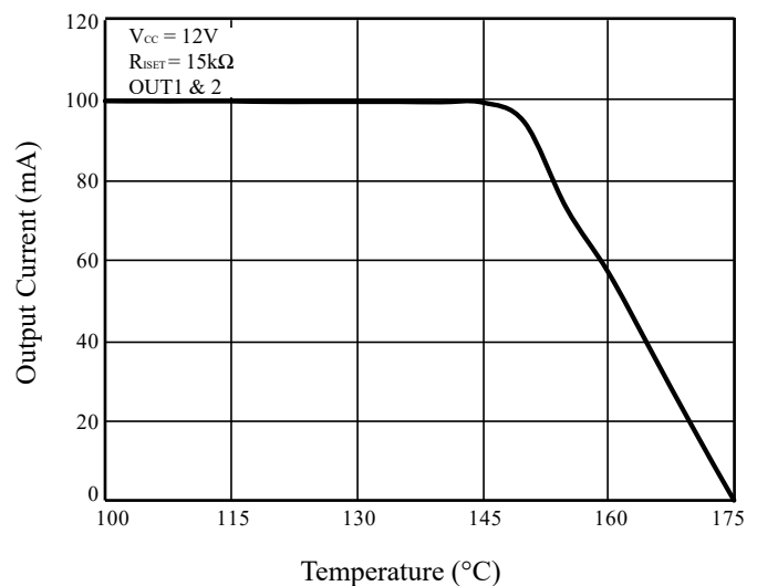
Figure 32 Thermal Roll Off
