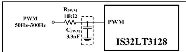
Figure 71 RC filter for PWM EMI
