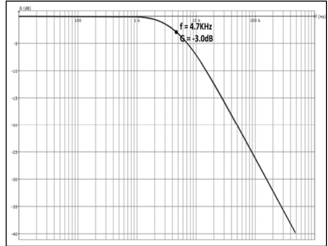
Figure 72 Low-Pass Filter Gain-Magnitude Frequency Response
