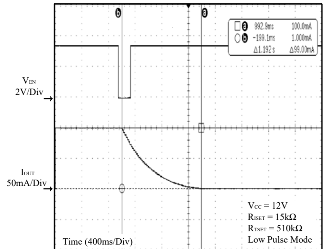
Figure 48 V_{EN} VS. I_{OUT}
