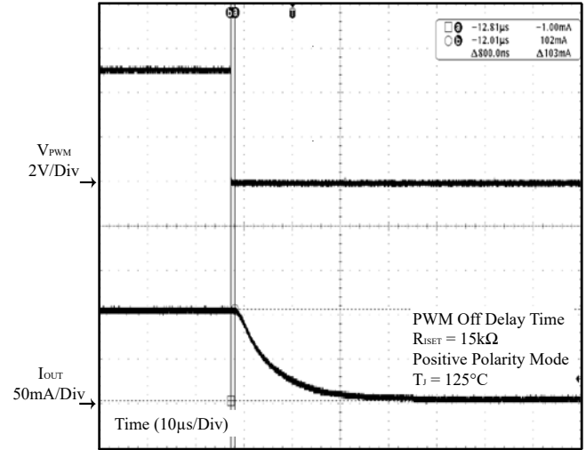
Figure 38 PWM Off Delay Time
