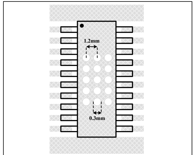
Figure 70 Board Via Layout For Thermal Dissipation
