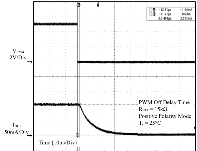
Figure 36 PWM Off Delay Time
