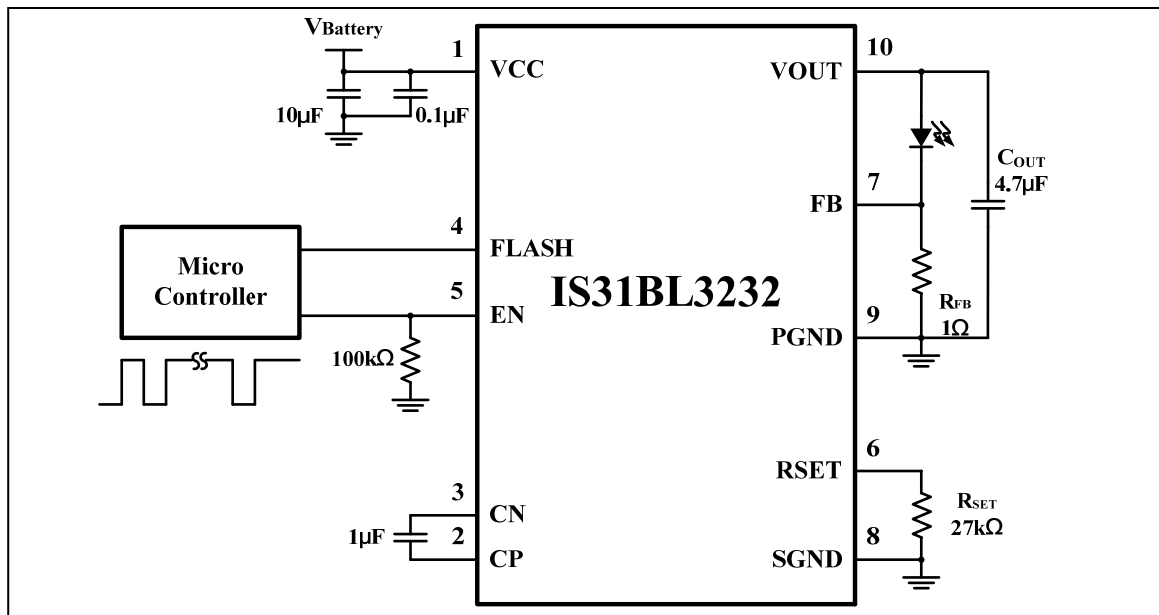
Figure 2 Typical Application Circuit (Torch Mode I_{V1} -50mA, Flash Mode 518mA)
