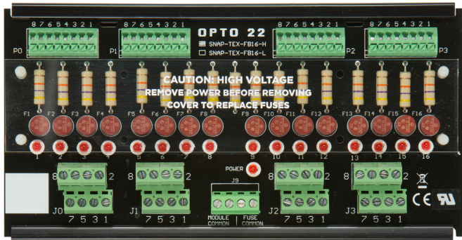
SNAP-TEX-FB16-H [Obsolete]
