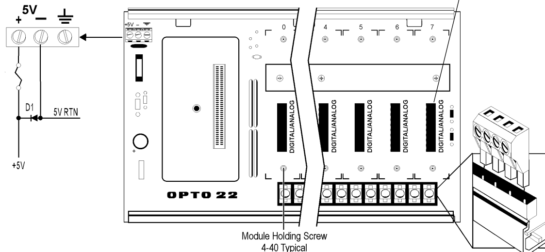
Power Schematic
