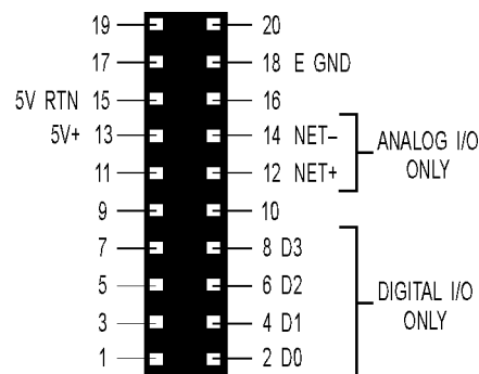
Module Mating Connector Pinout (female)
