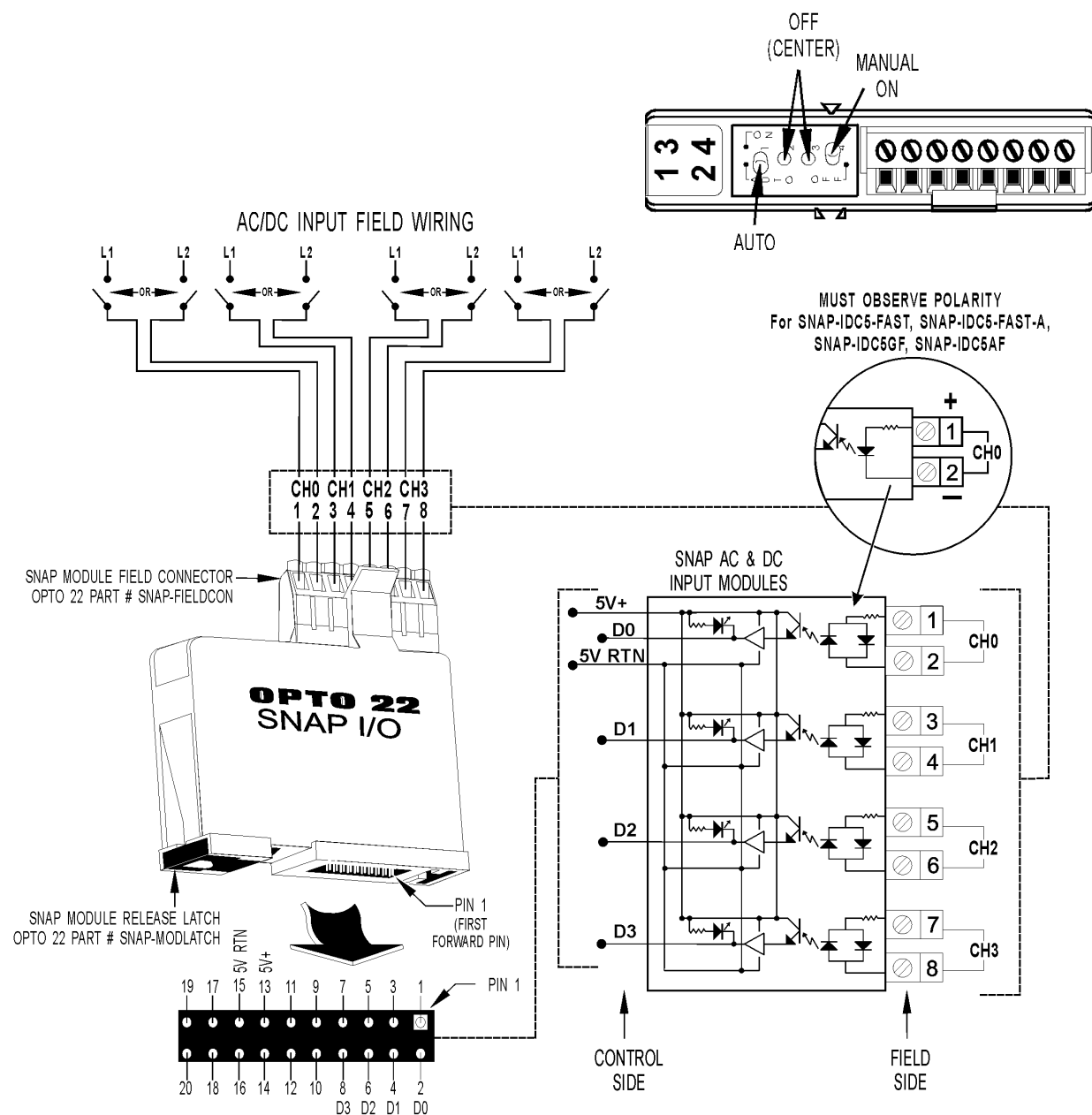
Snap Digital Module Base Control Connector (Bottom View)
