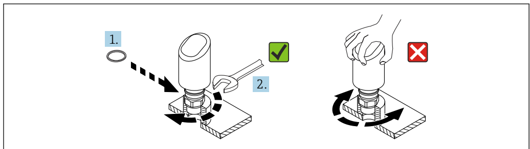
6 Screwing in the device
