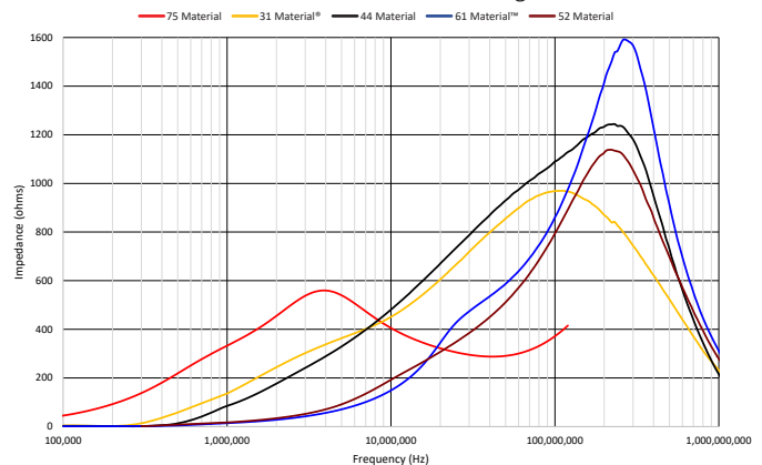
26XX801102 with 5 Turns 24 AWG Single Wire
