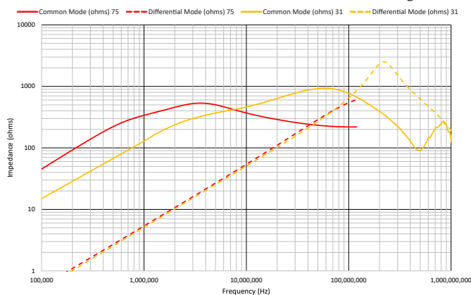
26XX801102 Differential with 5 Turns 24 AWG Sector Winding
