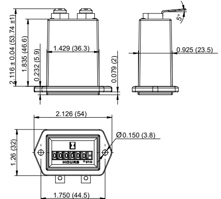
2-Hole w/glass lens and metal bezel
