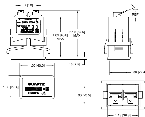
Flush-Rectangular
