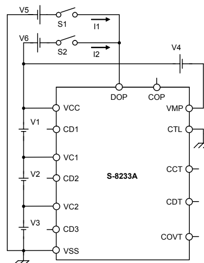
Test circuit 4
