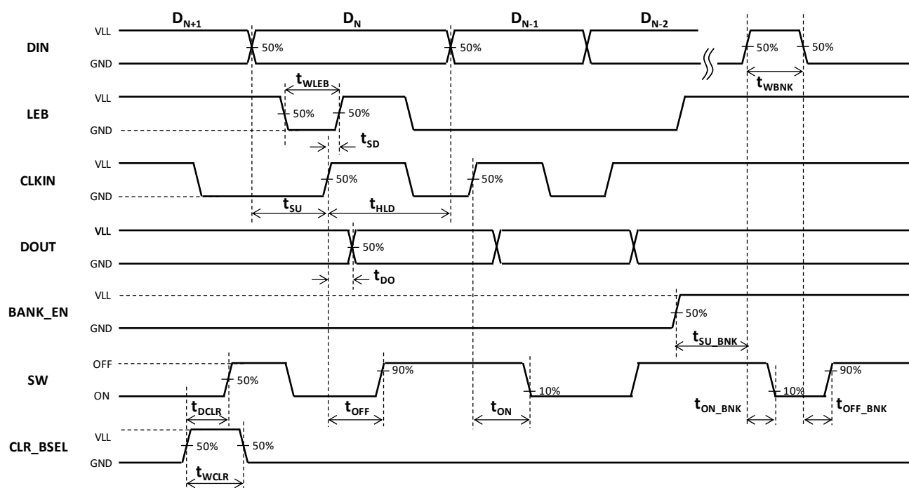
Figure 3 Logic Timing
