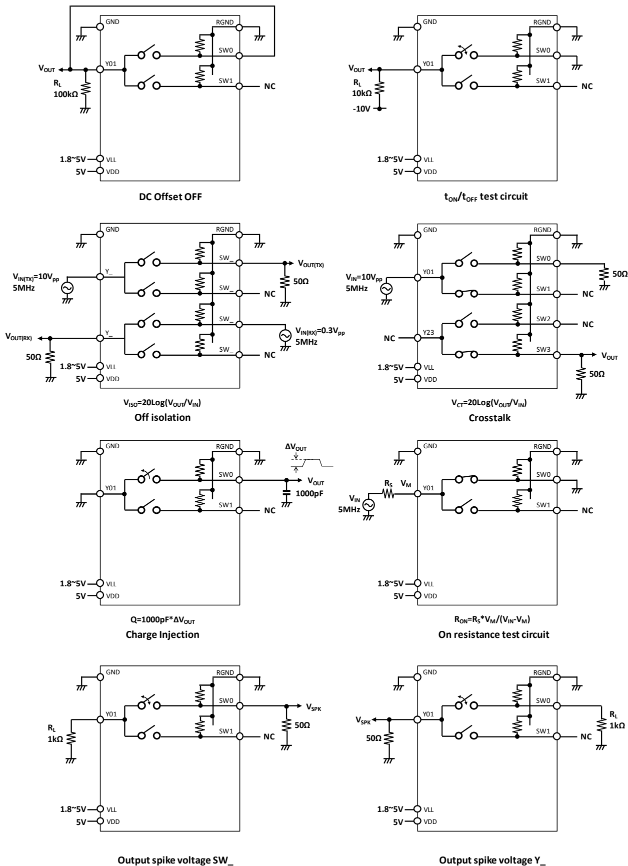
Figure 2 Test Circuits
