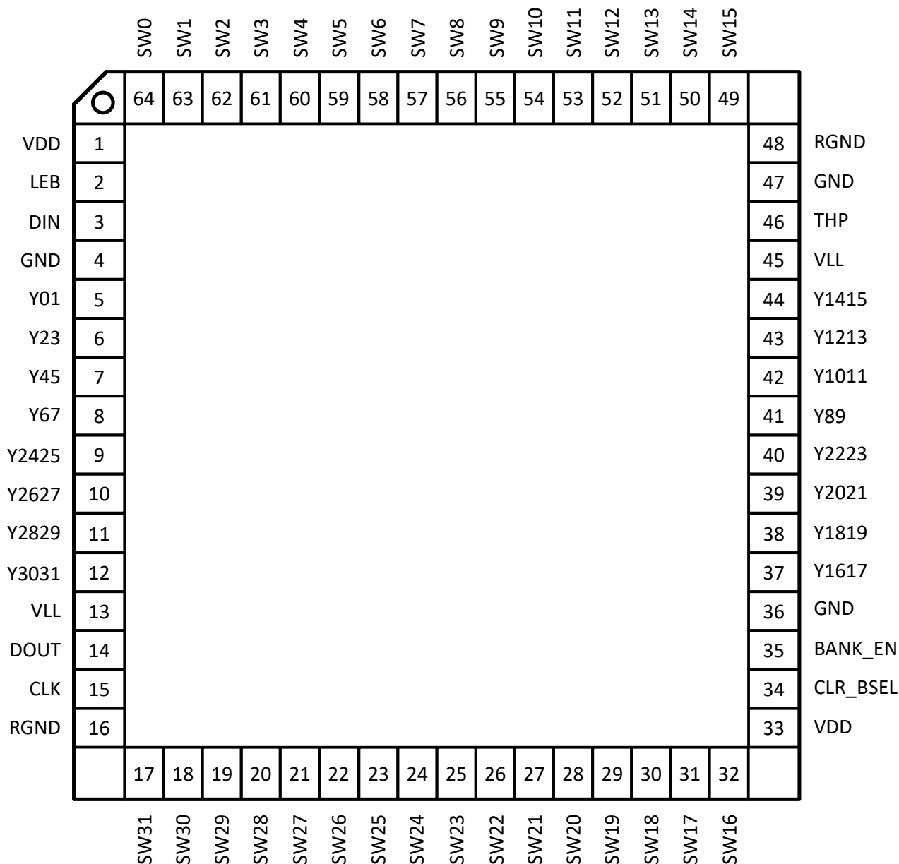
Figure 5 Pin Configuration
