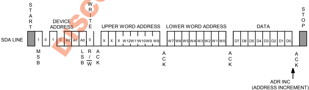
Figure 12 Byte Write
