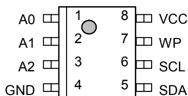
8-Pin SOP (JEDEC) Top view
