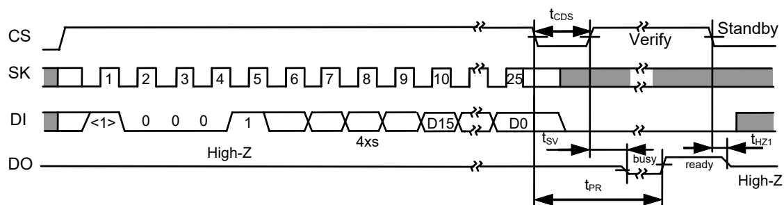
Figure 11 Chip Write Timing (S-93A46B)
