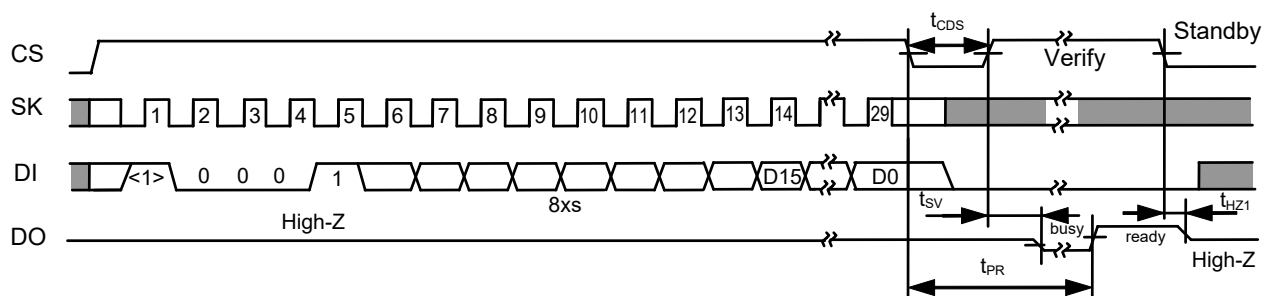
Figure 13 Chip Write Timing (S-93A76B/86B)
