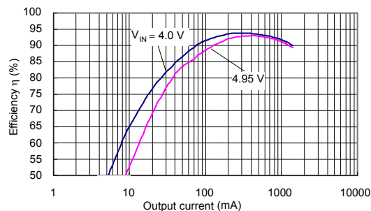
(6) S-8533A33AFT (Si3454DV/Si3455DV)
