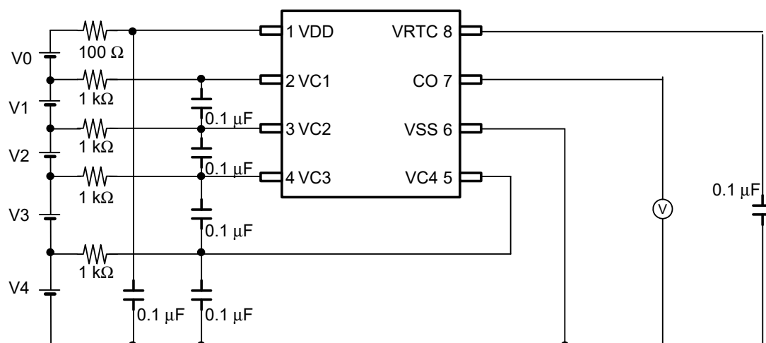
Figure 5 Test Circuit 1
