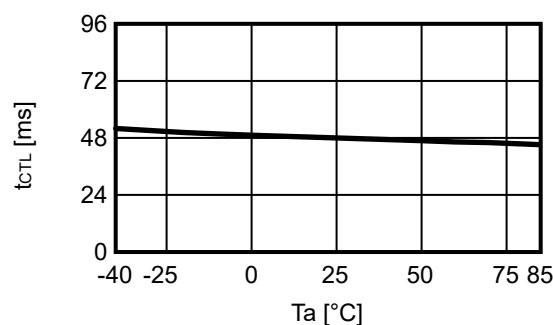
3. 12 t_{CTL} vs. T_a (S-82B2A Series)
