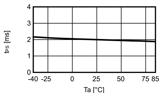
3. 14 t_{PS} vs. T_a (S-82B2B Series)
