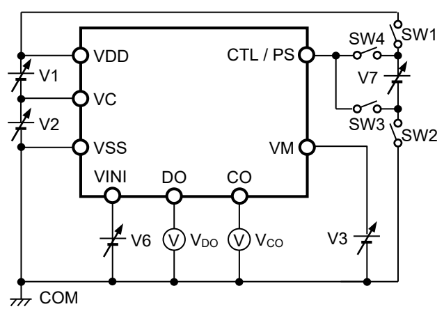
Figure 6 Test Circuit 2
