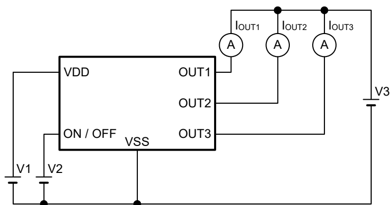
Figure 6 Test Circuit 3
