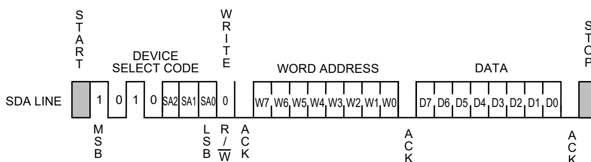
Figure 8 Byte Write
