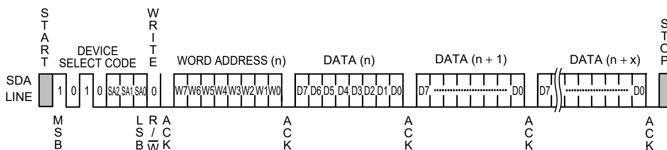
Figure 9 Page Write
