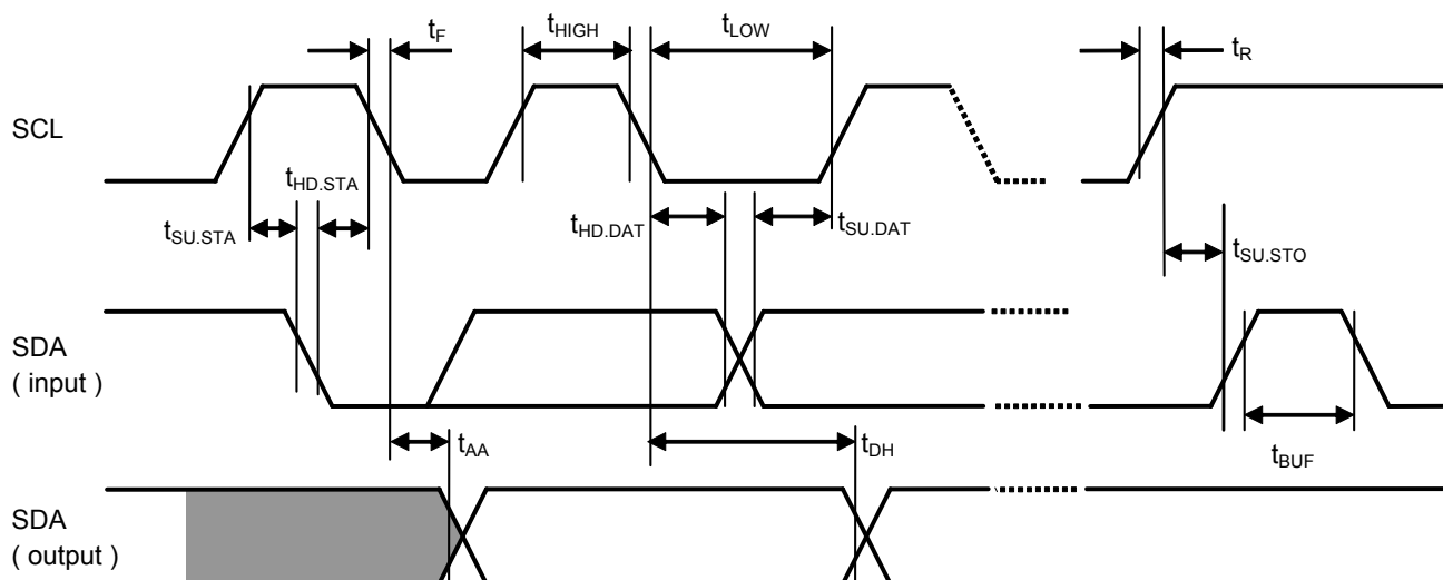
Figure 6 Bus Timing
