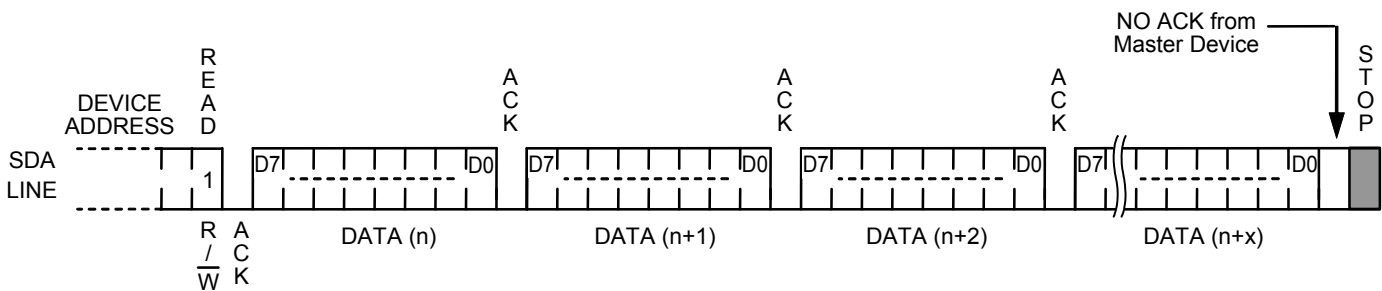
Figure 19 Sequential Read
