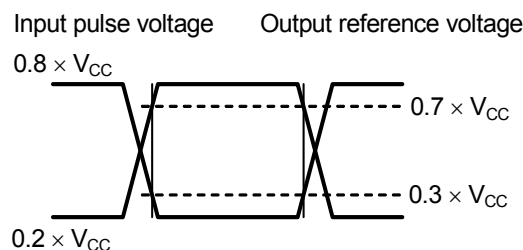
Figure 5 I/O Waveform during AC Measurement
