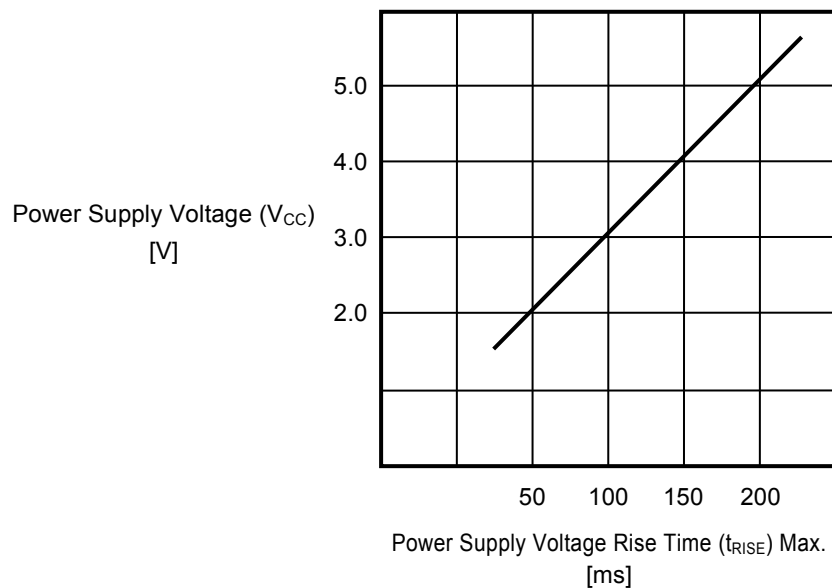
Figure 27 Power Supply Voltage Rise Time
