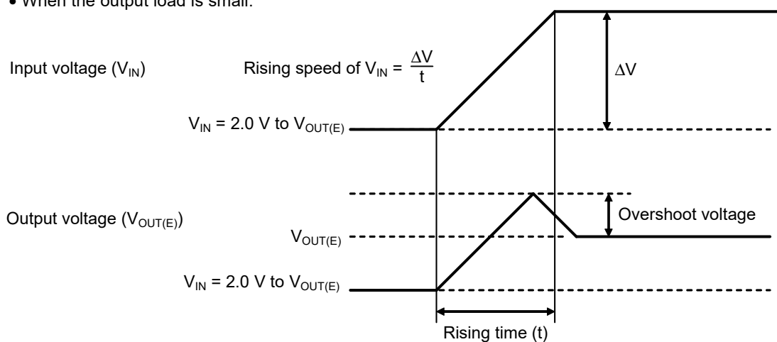
Figure 14 V_{IN} and Overshoot Voltage
