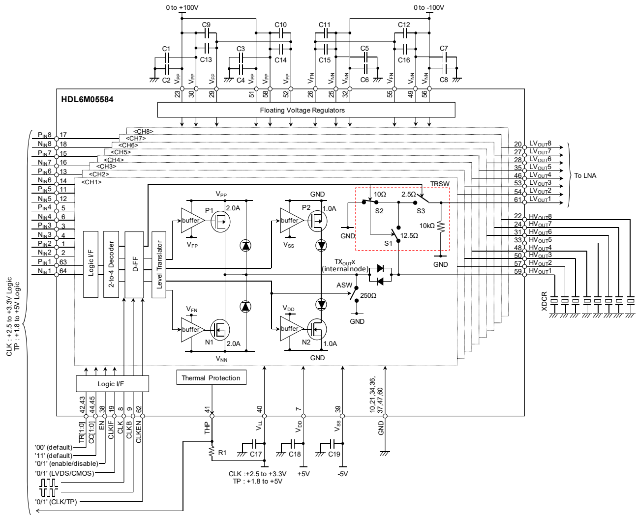
Fig.4 Typical Application Circuit
