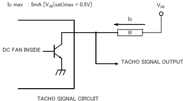
TACHO SIGNAL CIRCUIT
