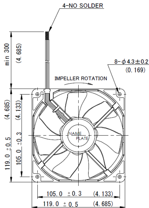
FLANGE TYPE
