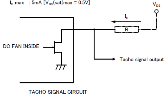
TACHO SIGNAL CIRCUIT
