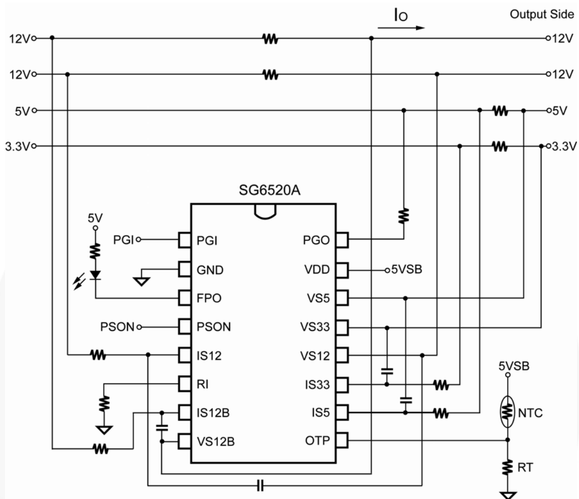
Figure 1. Typical Application
