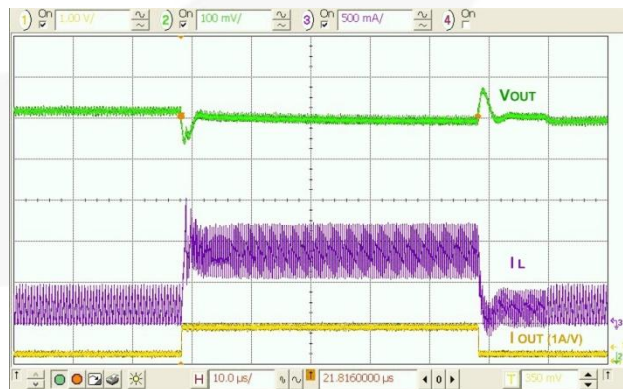
Figure 19. Load Transient, V_{IN}=5\text{ V} , V_{OUT}=3.3\text{ V} , 200-800-200 mA, 100 ns Edge
