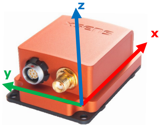
Figure 8: coordinate system of the enclosed MTi (Note: origin is located at the
