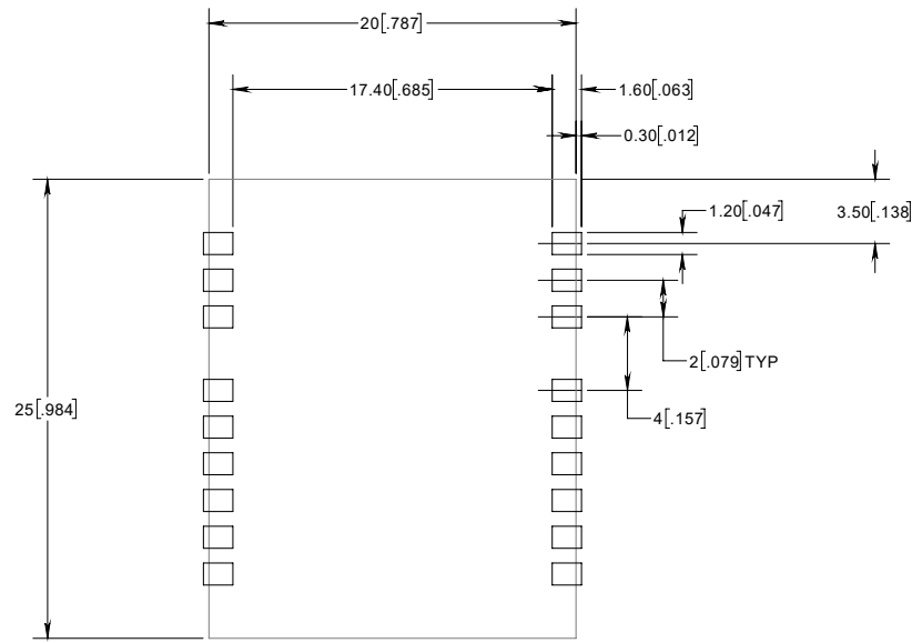
FOOTPRINT
