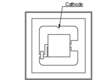
LED frontside view
