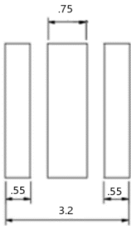
Suggested solder mask design
