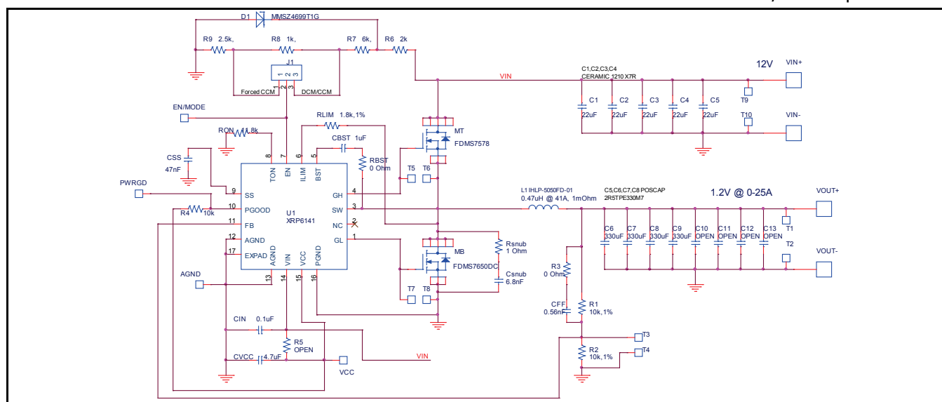
Fig. 1: XRP6141 Evaluation Board Schematics
