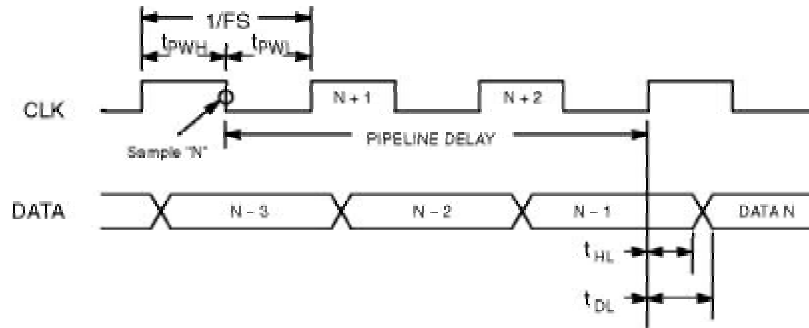
Figure 1. XRD8775 Timing Diagram
