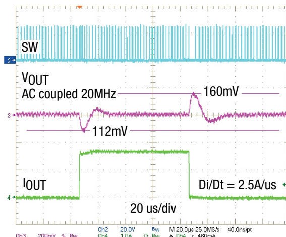
Figure 18. Load Step, CCM, 0\text{A}-1.5\text{A}-0\text{A}
