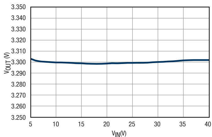
Figure 4. Line Regulation
