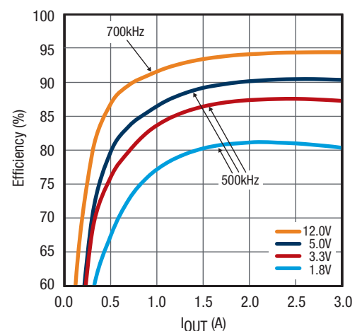
Figure 2. Efficiency, 24V_{IN}
