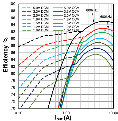
Figure 21: Efficiency, V_{\text{IN}}=12\text{V}
