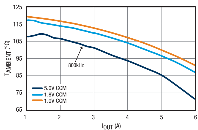
Figure 23. Maximum T_{\text{AMBIENT}} vs. I_{\text{OUT}} , V_{IN} = 12\text{V}
