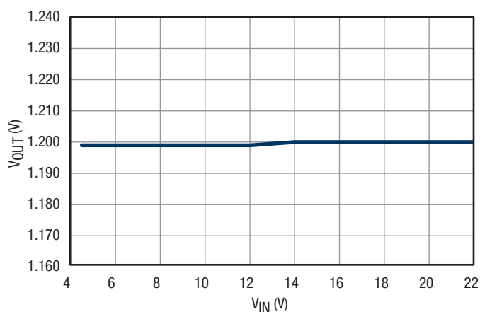
Figure 4. Line Regulation
