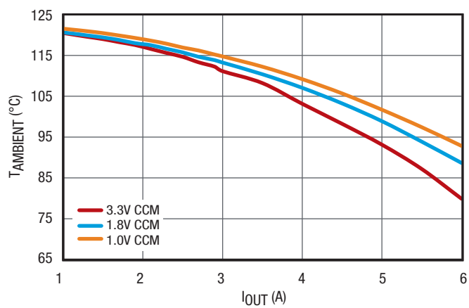
Figure 21. Maximum T_{\text{AMBIENT}} vs. I_{\text{OUT}} , V_{IN} = 5\text{V}
