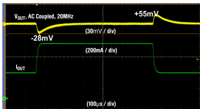
Figure 7. 5V IN , 1.1V OUT Transient Response, 0.5A to 1.0A
