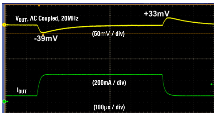
Figure 7. 5V IN , 1.1V OUT Transient Response, 0.5A to 1.0A
