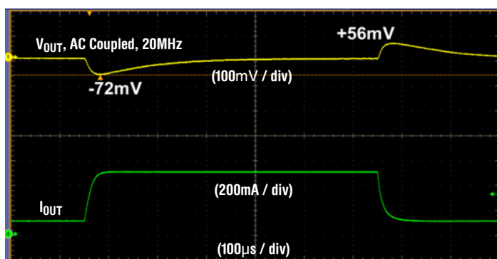
Figure 11. 5V IN , 3.3V OUT Transient Response, 0.1A to 0.5A
