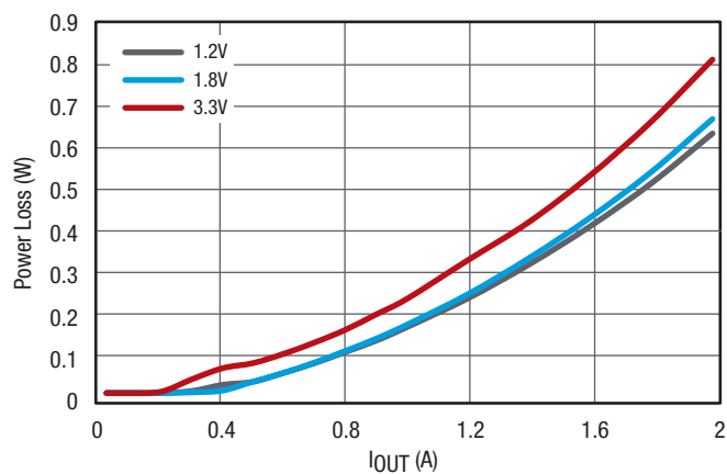
Figure 23. Channel 2 Power Loss at f_{SW} = 440\text{kHz} , V_{IN} = 12\text{V} , No Airflow
