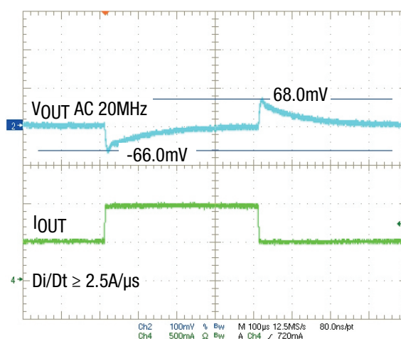
Figure 6. 5\text{V}_{\text{IN}} , 1.8\text{V}_{\text{OUT}} , f_{\text{SW}} = 440\text{kHz} Transient Response, 0.5A to 1.0A
