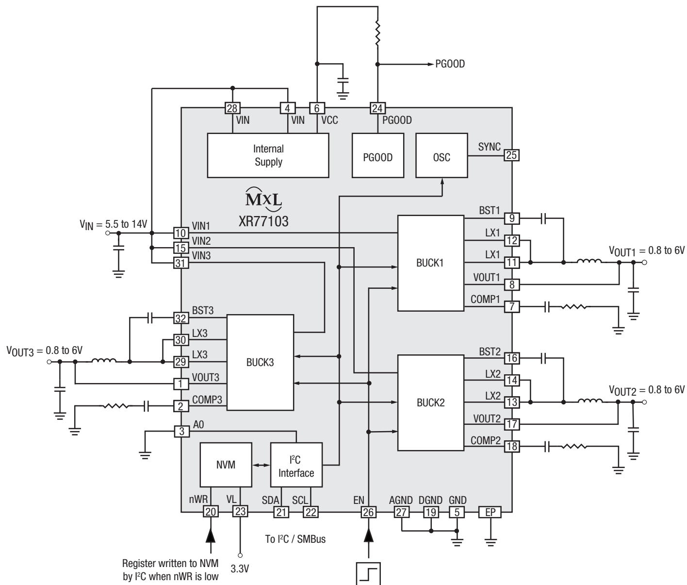
Figure 1. Typical Application
