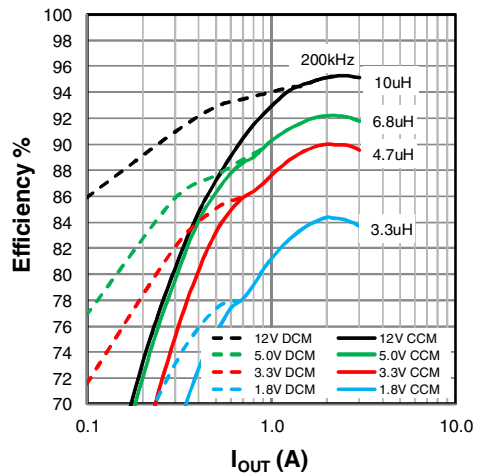
Figure 24: XR76203 Efficiency, V_{\text{IN}} = 24\text{V}
