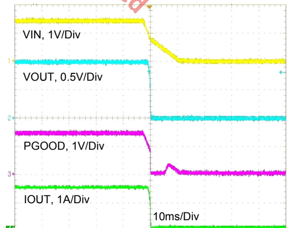
Figure 6: Powerdown, IOUT=1.5A, 1.5VIN, 1VOUT
