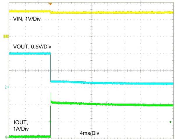
Figure 2: Short-circuit, 1.5VIN, 1VOUT
