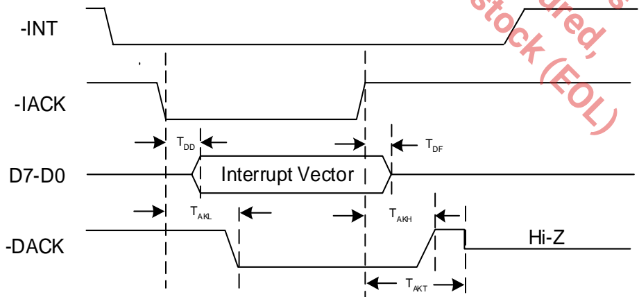
Figure 7: Interrupt Timing
