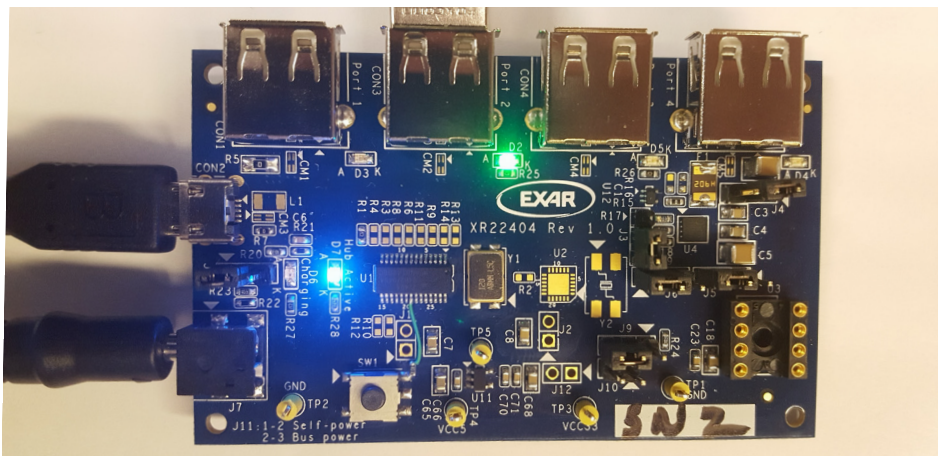
Figure 2: XR22404 PCB
