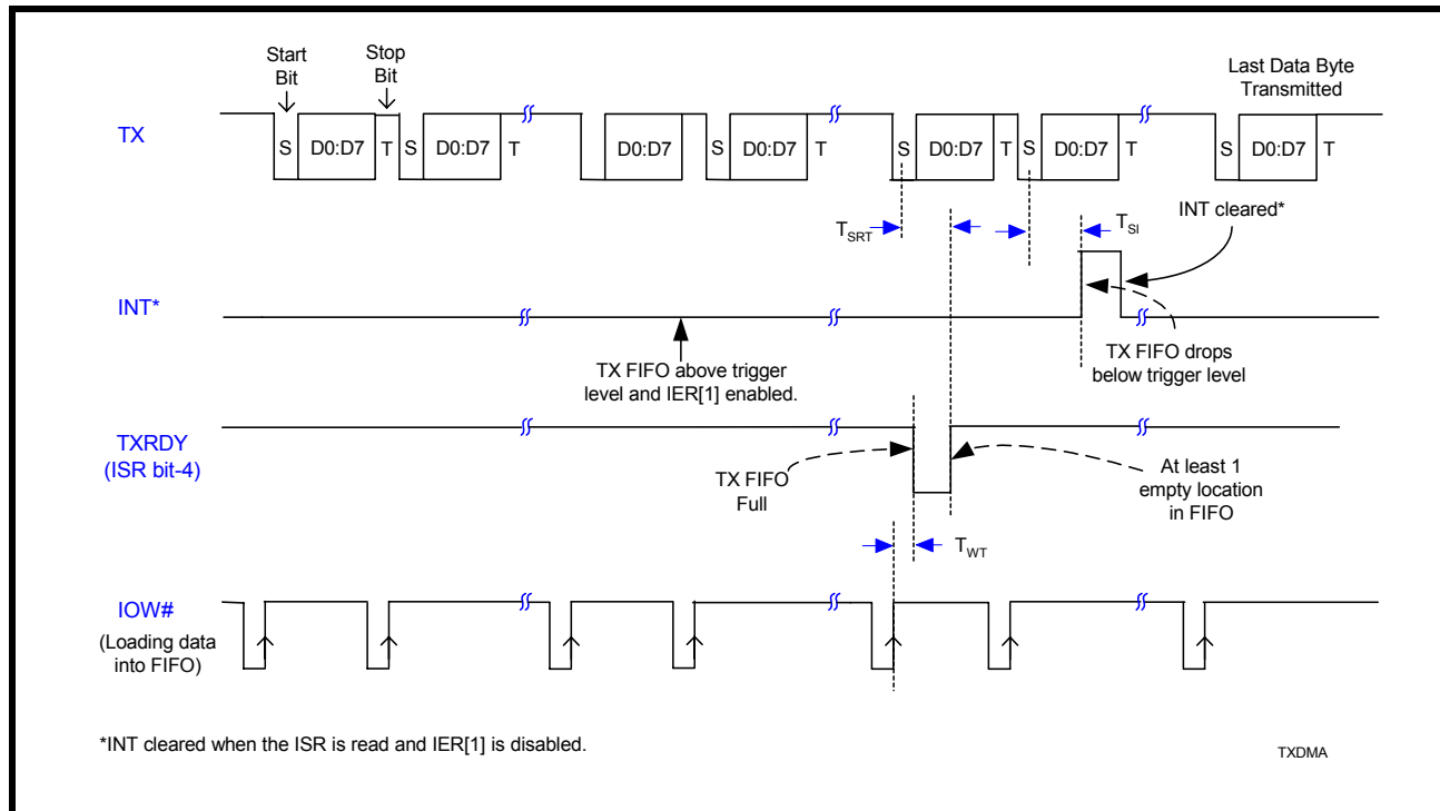
FIGURE 17. TRANSMIT READY & INTERRUPT TIMING [FIFO MODE, DMA MODE ENABLED]
