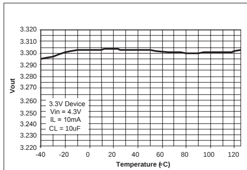
Figure 10. Output Voltage vs Temperature at I_{LOAD}=10mA
