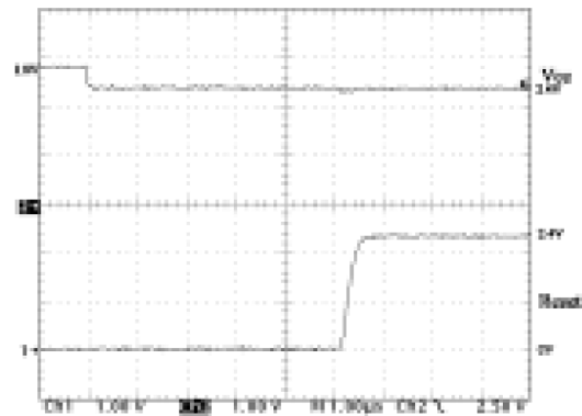
Figure 16: SP708 RESET Response Time
