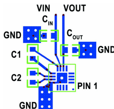
Figure 4: PCB Lay-out
