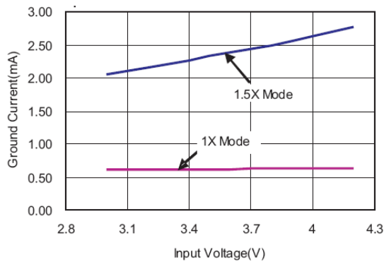
5. Ground Current vs Input Voltage
