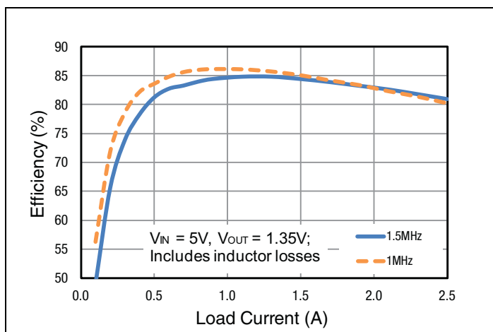
Figure 5: Buck 3 Efficiency
