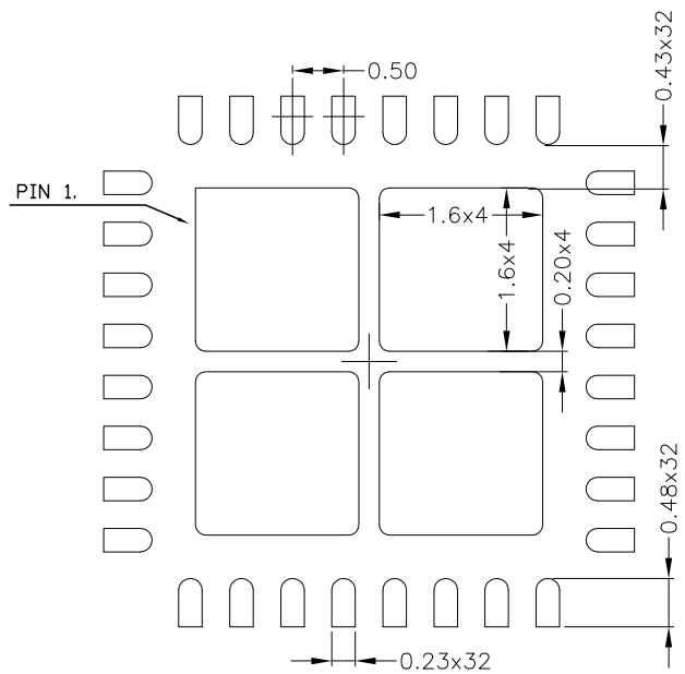
TYPICAL RECOMMENDED STENCIL
