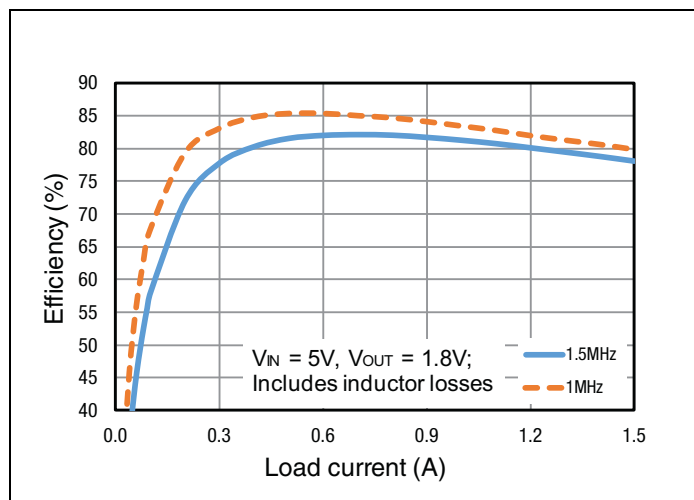
Figure 4: Buck 2 Efficiency
