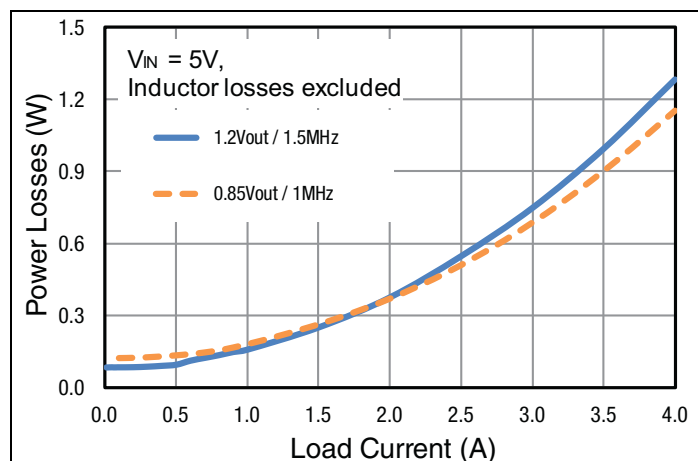
Figure 12: Buck 4 Power Loss
