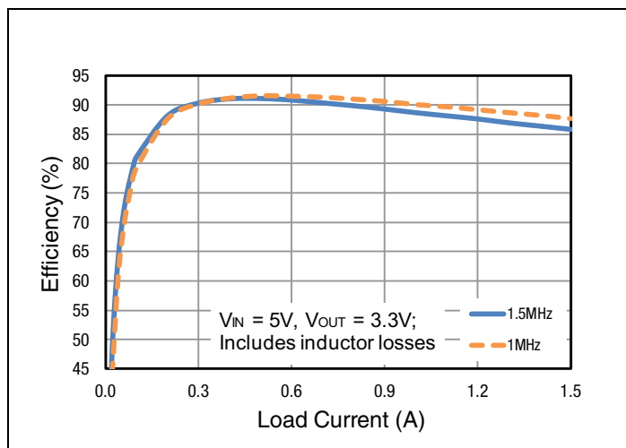
Figure 3: Buck 1 Efficiency
