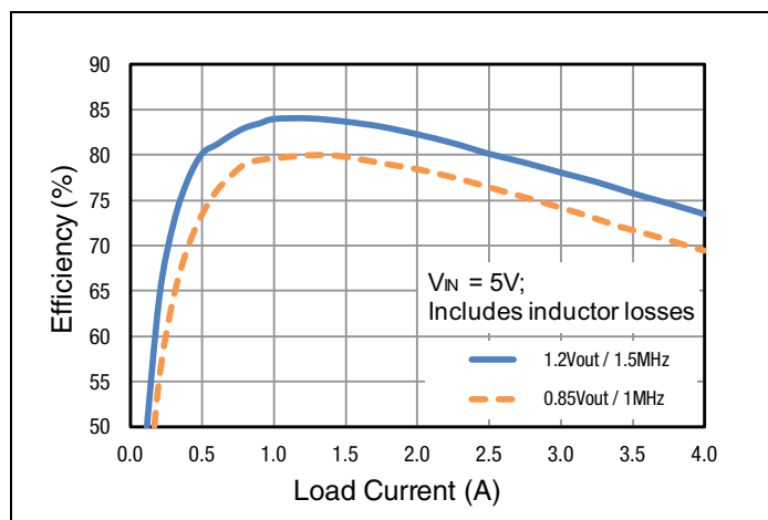
Figure 6: Buck 4 Efficiency
