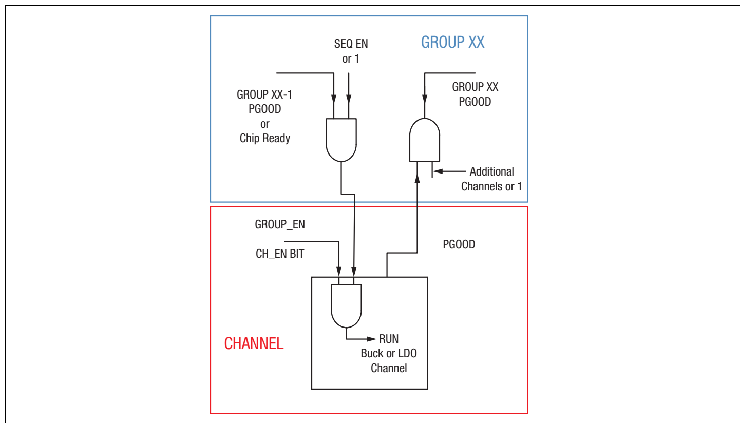
Figure 15: Sequencing
