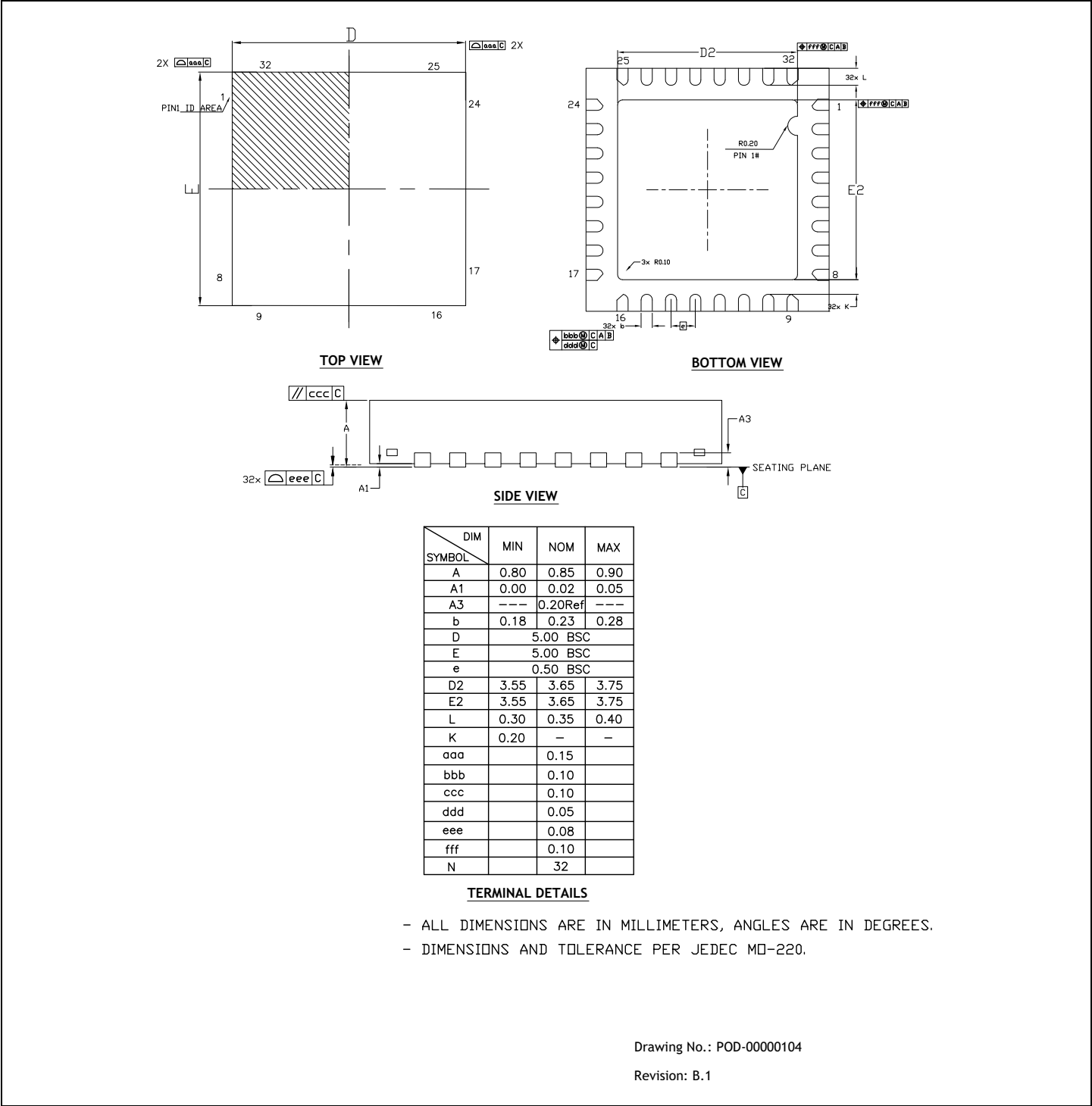
Figure 20: Mechanical Dimensions
